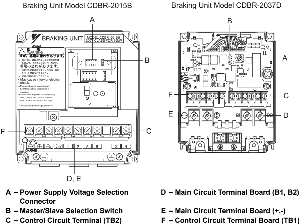
Figure 1 CDBR-□□□□B to CDBR-□□□□D Front View
