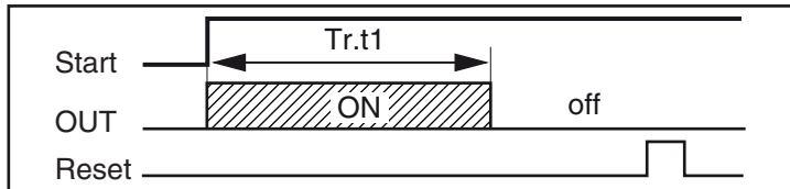
Asymmetrical oscillator with start in OFF.
