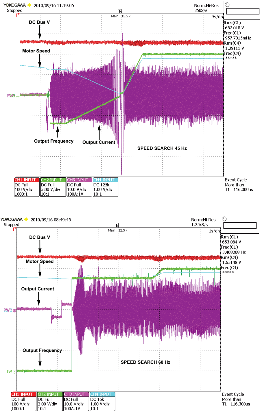
Figure 7 Bi-Directional Speed Search
