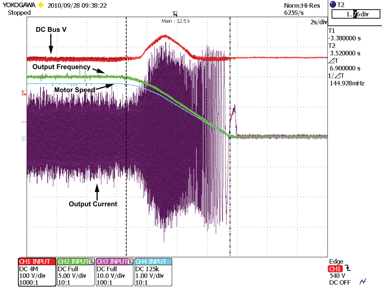
Figure 5 Over-Excitation Braking
