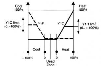
Fig. 1: Output characteristic for dual action controllers. Example: Heat - Cool
